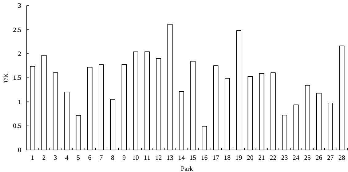
图 3 绿地公园内部平均温度与周围 500 m 平均温度对比 Fig. 3 The internal temperature compared with the temperature of around 500 m
