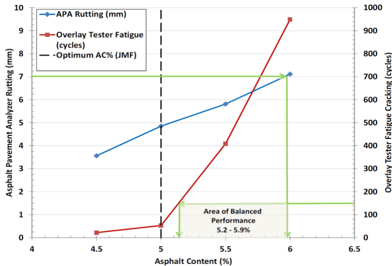
Figure 5 – Balanced Mixture Design Process for a 9.5mm NMA Asphalt Mixture Using a PG64S-22 Asphalt Binder
