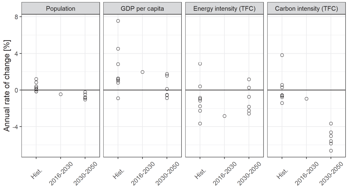
Figure 3 Annual change rate in major drivers of emissions. “Hist” are values for eight timeframes between 1960-2016. “2016-2030” are based on NDC assumptions. “2030-2050” are values for Japan 80% emissions reduction scenario from six different models. Based on data from Kuriyama et al. (Energy Policy 2019) and Sugiyama et al. (Energy 2019).
