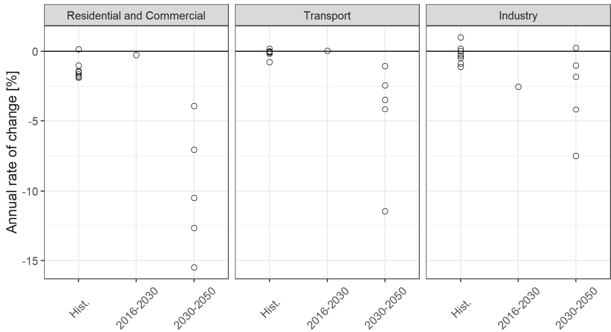
Figure 4 Annual change rate in carbon intensity of energy consumption by aggregated economic sectors. “Hist” are values for eight timeframes between 1960-2016. “2016-2030” are based on NDC assumptions. “2030-2050” are values for Japan 80% emissions reduction scenario from six different models. Based on data from Kuriyama et al. (Energy Policy 2019) and Sugiyama et al. (Energy 2019).
